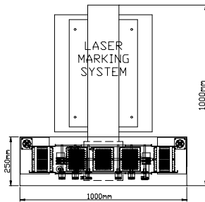
KH8300 Pallet Auto-loader
